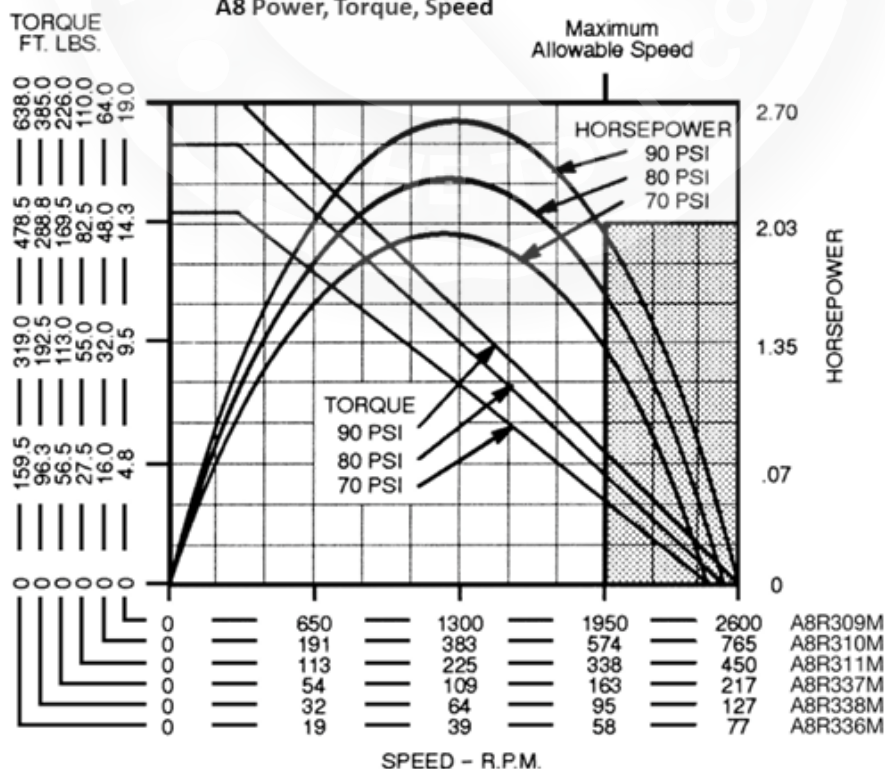
A8 Power, Torque, Speed
